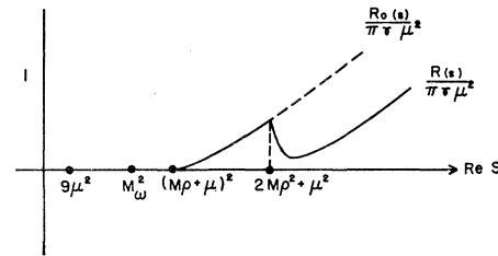
FIG. 5. \rho - \pi phase space with and without recoupling.
