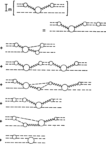
FIG. 3. Contributions of elastic unitarity.
